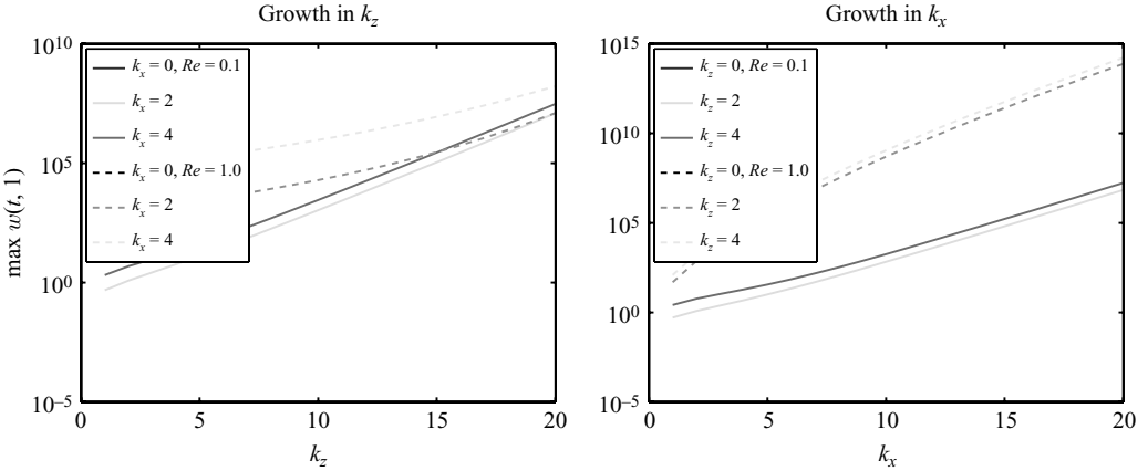
FIGURE 9. \max_t \{|W^r|_{y=1}\} growing in k_z and k_x forced by u'_y|_{y=0} = \sin(t) .
