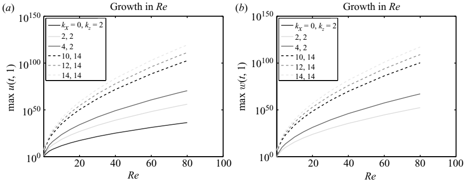
FIGURE 10. (a) \max_t \{|u^r|_{y=1}\} and (b) \max_t \{|W^r|_{y=1}\} growing in Re forced by u'_y|_{y=0} = \sin(t) .
