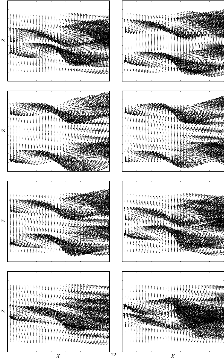
FIGURE 4. Snapshots of the desired skin friction spatio-temporal profile (reference output trajectory). Time proceeds left to right and top to bottom. Arrows indicate direction and magnitude.
