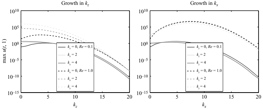
FIGURE 14. \max_t\{|u'|_{y=1}|\} growing in k_z and k_x forced by p^r|_{y=0} = (1/\pi^3)e^{-(k_x^2/\pi^2 - k_z^2/\pi^2)} \sin(t) .
